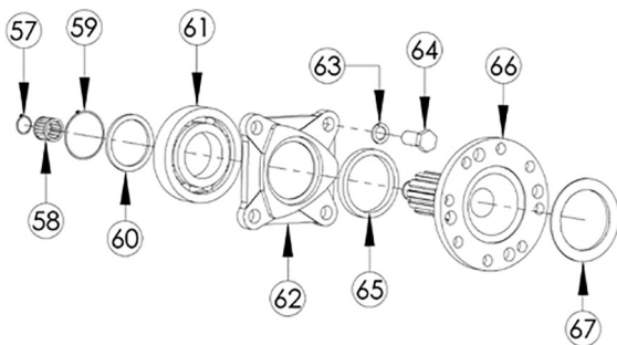
Detail F – 1410 Output Flange Kit – Option “C” SSH2 - 14/21 & SSV* - 14/21 Part No: 2053490000
