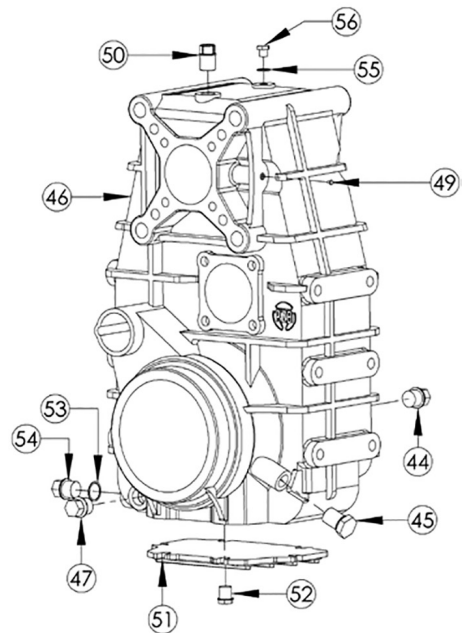
Detail E – SSV Housing
