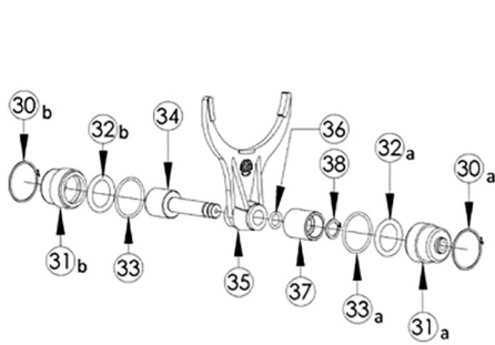
Detail C – SSH2/SSV* - 14/21 Shift Cylinder Assembly
