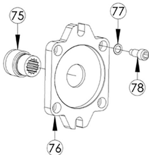
Detail F – SAE “C” (2-Bolt) – Option “E” SSH2 - 14/21 & SSV* - 14/21 Part No: 2054260000
