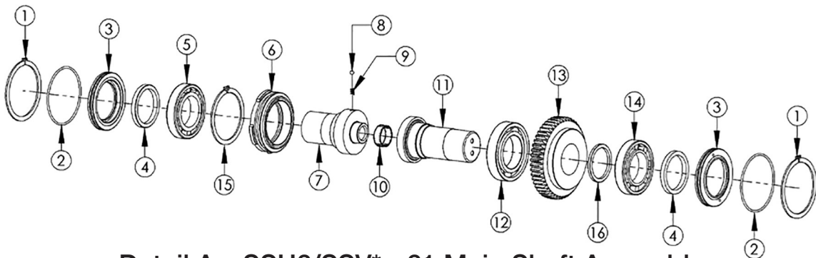
Detail A – SSH2/SSV* - 21 Main Shaft Assembly
