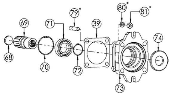
Detail F – SAE “B-B” Hyd. Flange – Option “P” SSH2 - 14/21 & SSV* - 14/21 Part No: 35205200008
