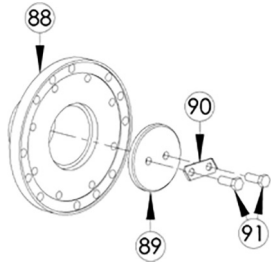
Detail G – Main Shaft Flange Kit (1610/1710/1810) SSH2 & SSV* - 21 Part No: 205F7860000
