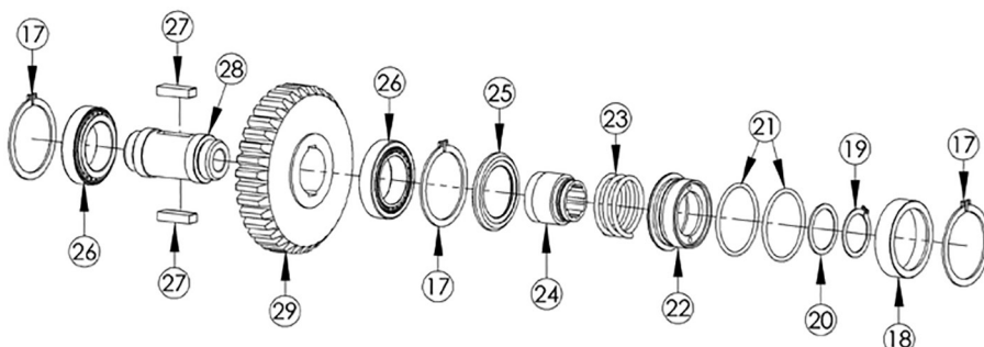
Detail B – SSV4 - 14/21 Main Shaft Assembly
