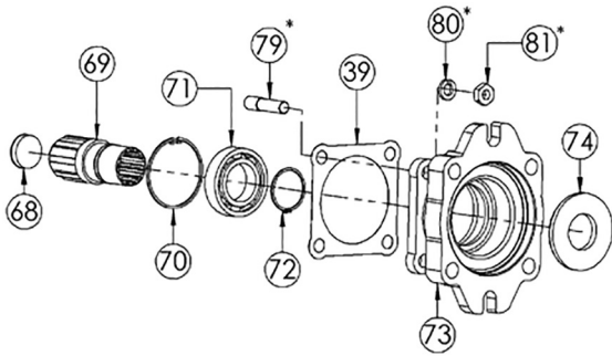
Detail F – SAE “B” Hyd. Flange – Option “K” SSH2 - 14/21 & SSV* - 14/21 Part No: 35205100008
