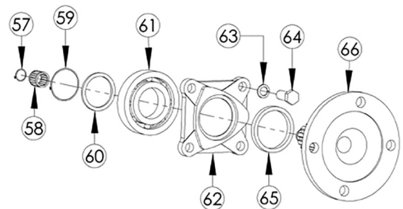
Detail F – 1500 Output Flange Kit – Option “D” SSH2 - 14/21 & SSV* - 14/21 Part No: 2053640000
