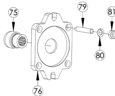
Detail F – SAE “C” (4-Bolt) – Option “E” SSH2 - 14/21 & SSV* - 14/21 Part No: 2054260000
