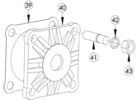
Detail D – SSH2/SSV* Cover Assembly
