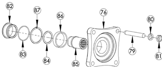
Detail F – SAE “D” Hyd. Flange – Option “H” SSV* - 14/21 Part No: 2054280000
