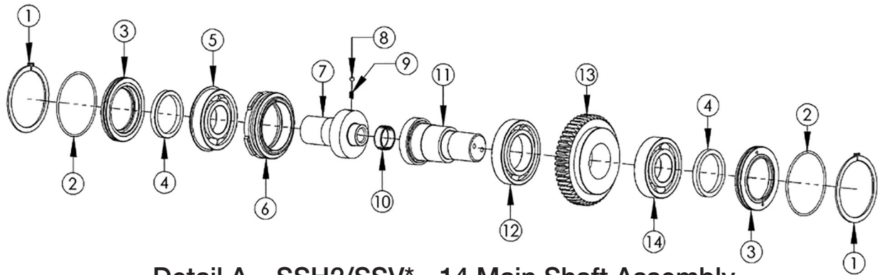
Detail A – SSH2/SSV* - 14 Main Shaft Assembly
