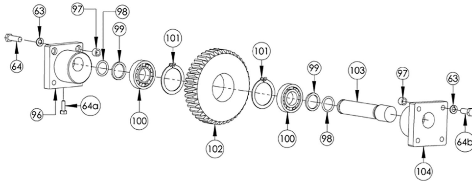
Detail H – SSV4 - 14/21 Auxiliary Shaft
