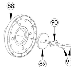
Detail G – Main Shaft Flange Kit (1550/1610/1710/1810) SSH2 & SSV* - 14 Part No: 205F8330000
