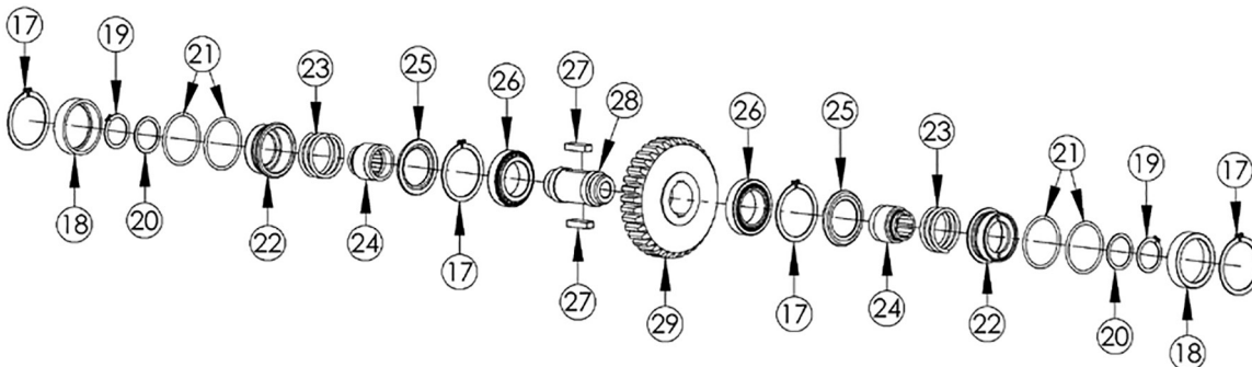
Detail B – SSH2/SSV* - 14/21 Main Shaft Assembly
