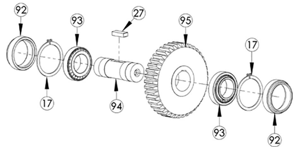
Detail H – SSV -14/21 Auxiliary Shaft
