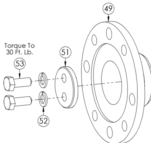
SS66 – 1480/1550 Flange
