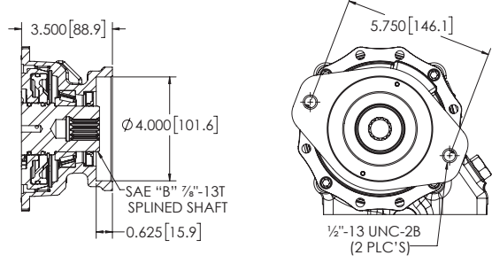
"BS" OUTPUT - SAE "B" 7/8" -13T SHAFT SAE "B" 2-BOLT
