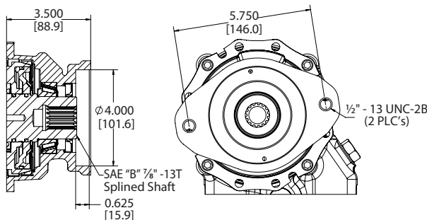
"B6" OUTPUT - Special SAE "B" 7/8" -13T, 2-Bolt SAE "B"
