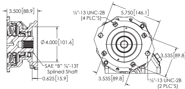
"BB" OUTPUT - SAE "B" 7/8" -13T, 2- & 4-BOLT SAE-"B"
