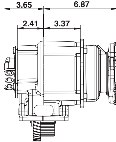
MC1 w/Remote Solenoid
