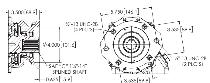
"CB" OUTPUT - SAE "C" 1 1/4" -14T, SAE "B" NOTE: Only used with extended shaft.
