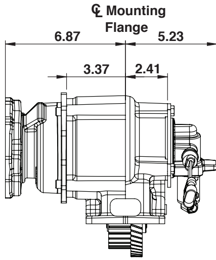
MC1 w/Integral Solenoid
