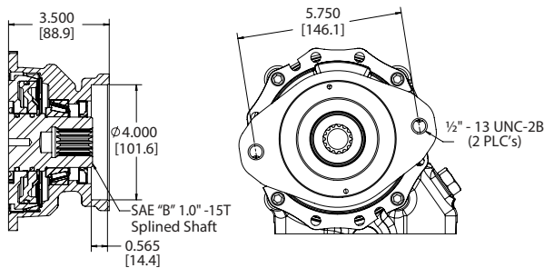
“P6” OUTPUT - SAE “BB” 1.0" -15T, 2-BOLT SAE “B Special”
