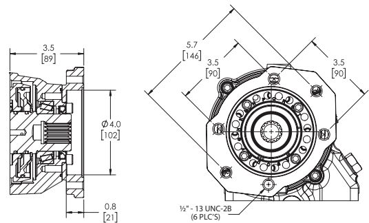
"BB" OUTPUT – SAE "B" 7/8"-13T, SAE "B" 2- & 4-Bolt
